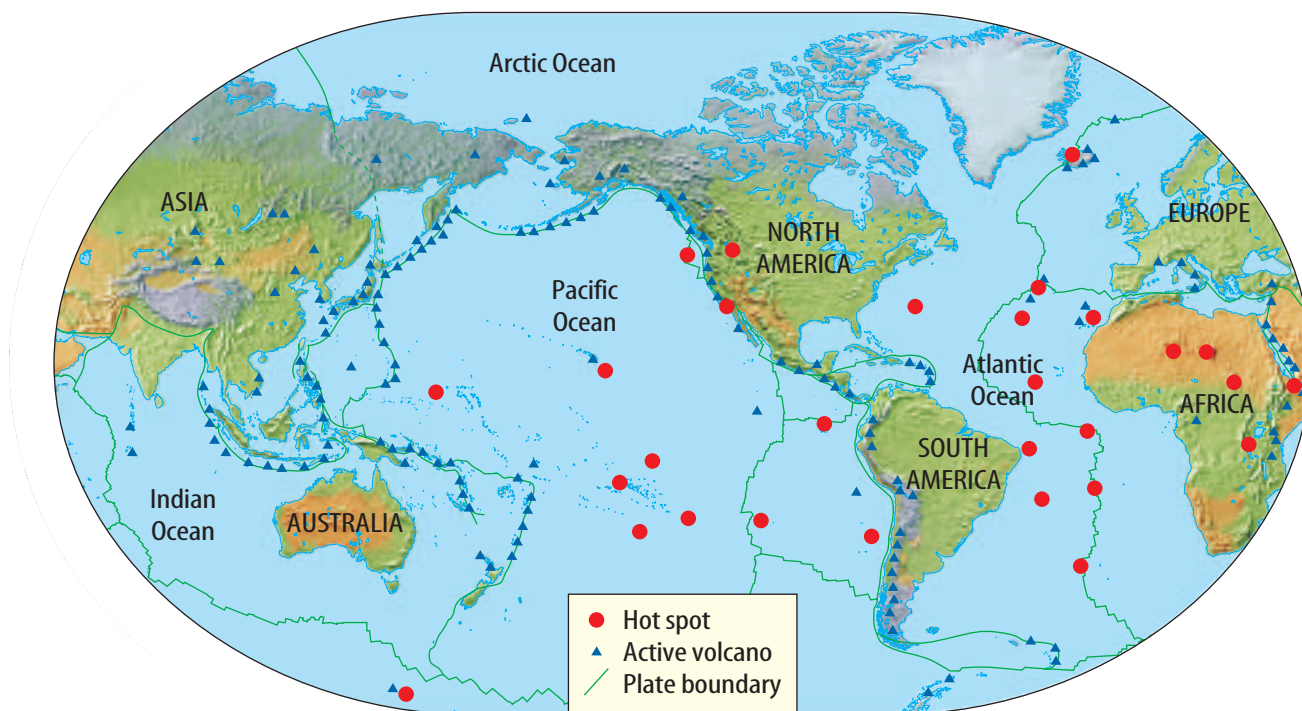
Figure 5 This map shows the locations of volcanoes, hot spots, and plate boundaries around the world. The Ring of Fire is a belt of active volcanoes that circles the Pacific Ocean.
