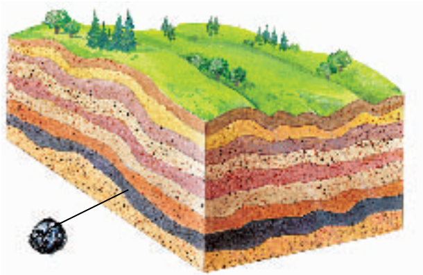
D When bituminous coal is heated and squeezed during metamorphism, anthracite coal forms.
