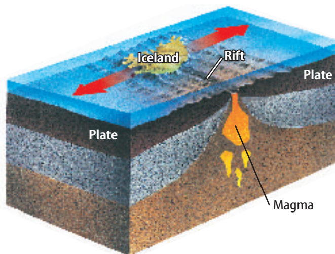
Figure 6 This diagram shows how volcanic activity occurs where Earth's plates move apart.
