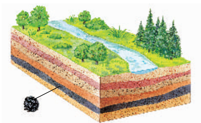
C As the lignite coal becomes buried by more sediments, heat and pressure change it into bituminous coal.
