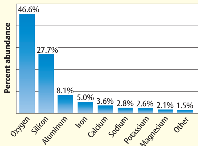
Figure 5 Most of Earth's crust is composed of eight elements.
